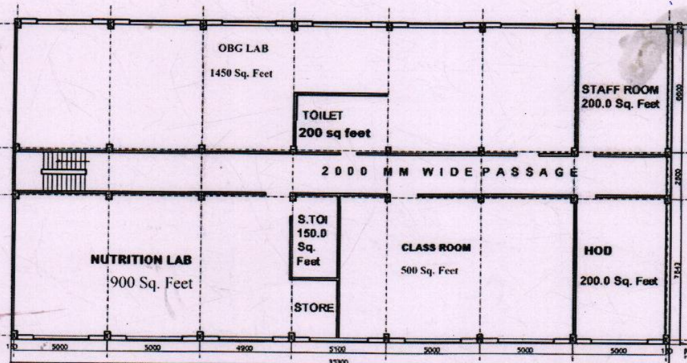
SECOND FLOOR PLAN (BLOCK - A)
